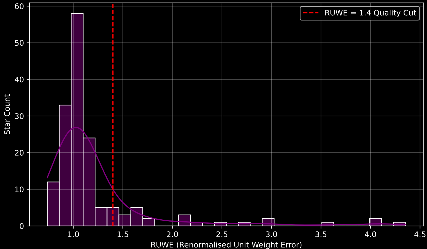
GAPOGEE DR17 Field [272-22-O_TESS] RUWE Distribution (n= 159)
