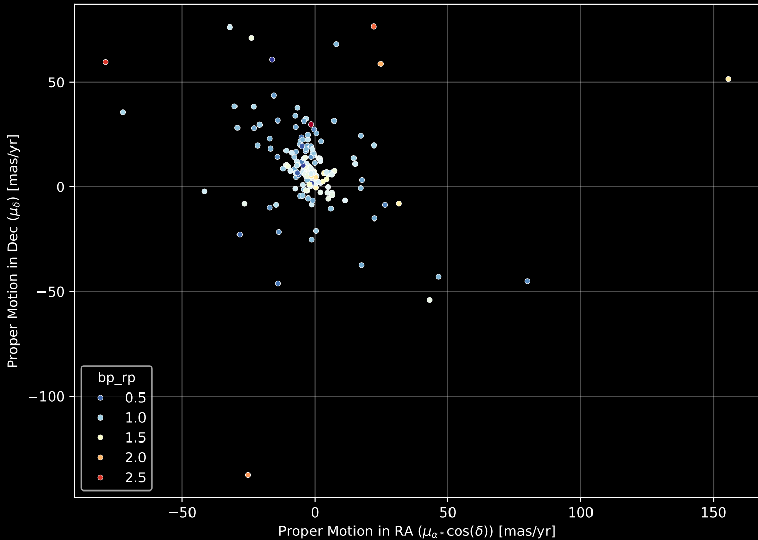
APOGEE DR17 Field: [272-22-O_TESS] Proper Motion Diagram (n= 163)
