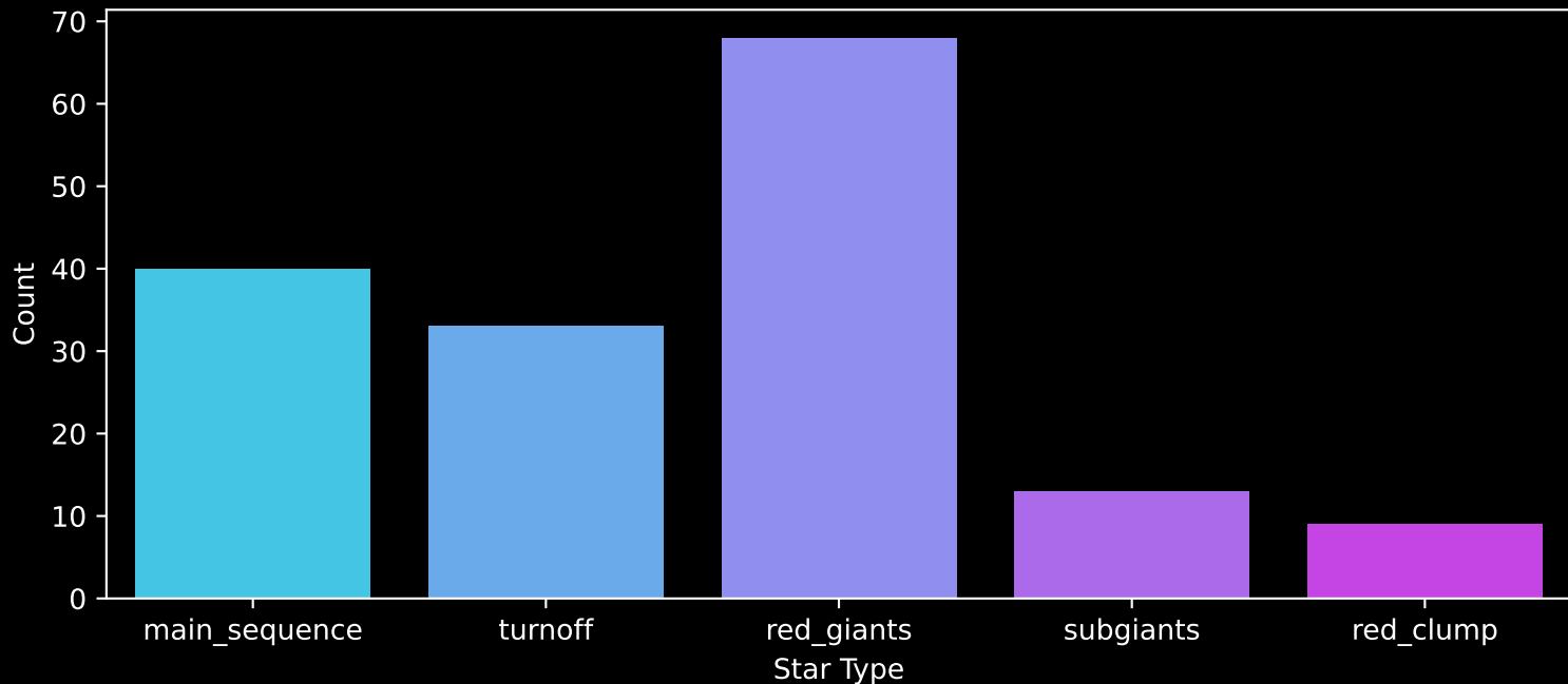
APOGEE DR17 Field: [272-22-O_TESS] Count plot of Star Type
