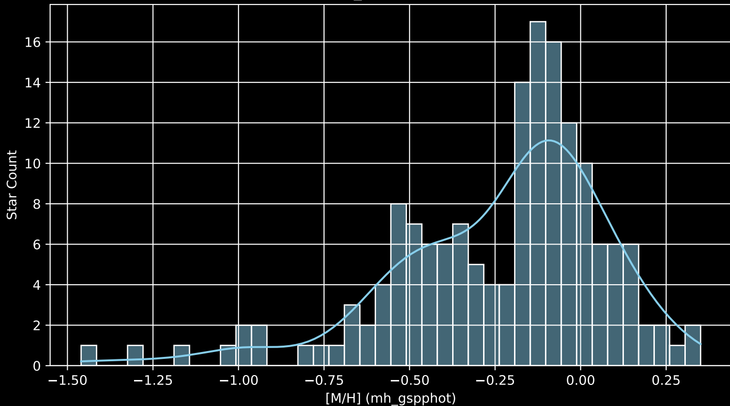
APOGEE DR17 Field: [272-22-O_TESS [M/H] (mh_gspphot) (n= 161)
