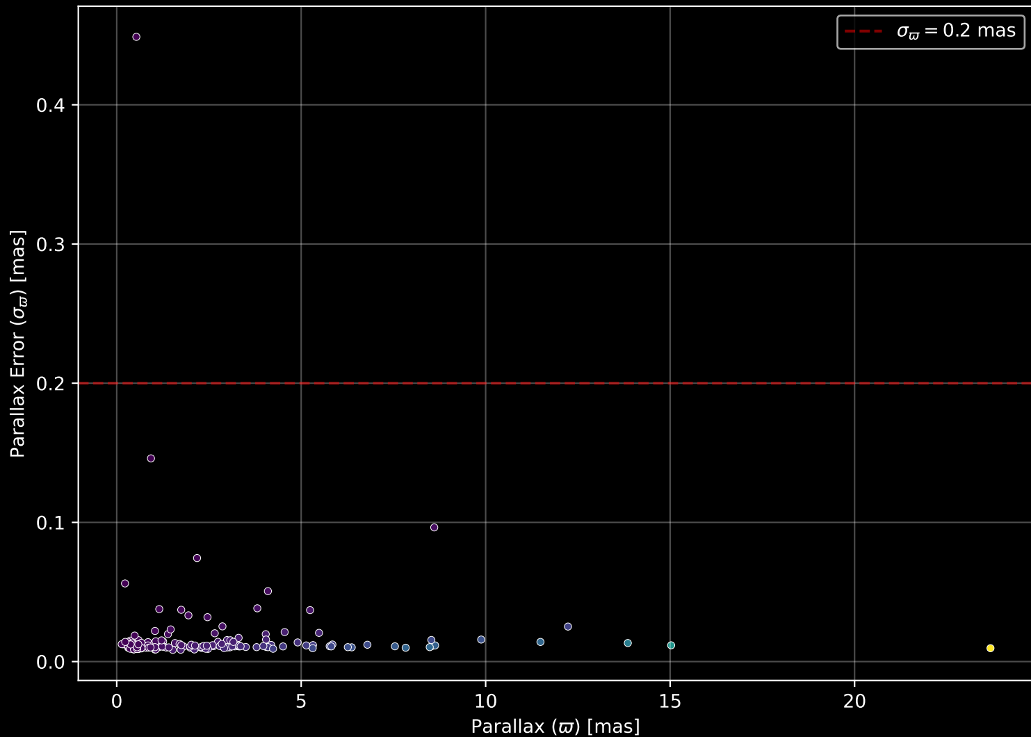
APOGEE DR17 Field: [272-22-O_TESS] Parallax Quality (n= 163)
